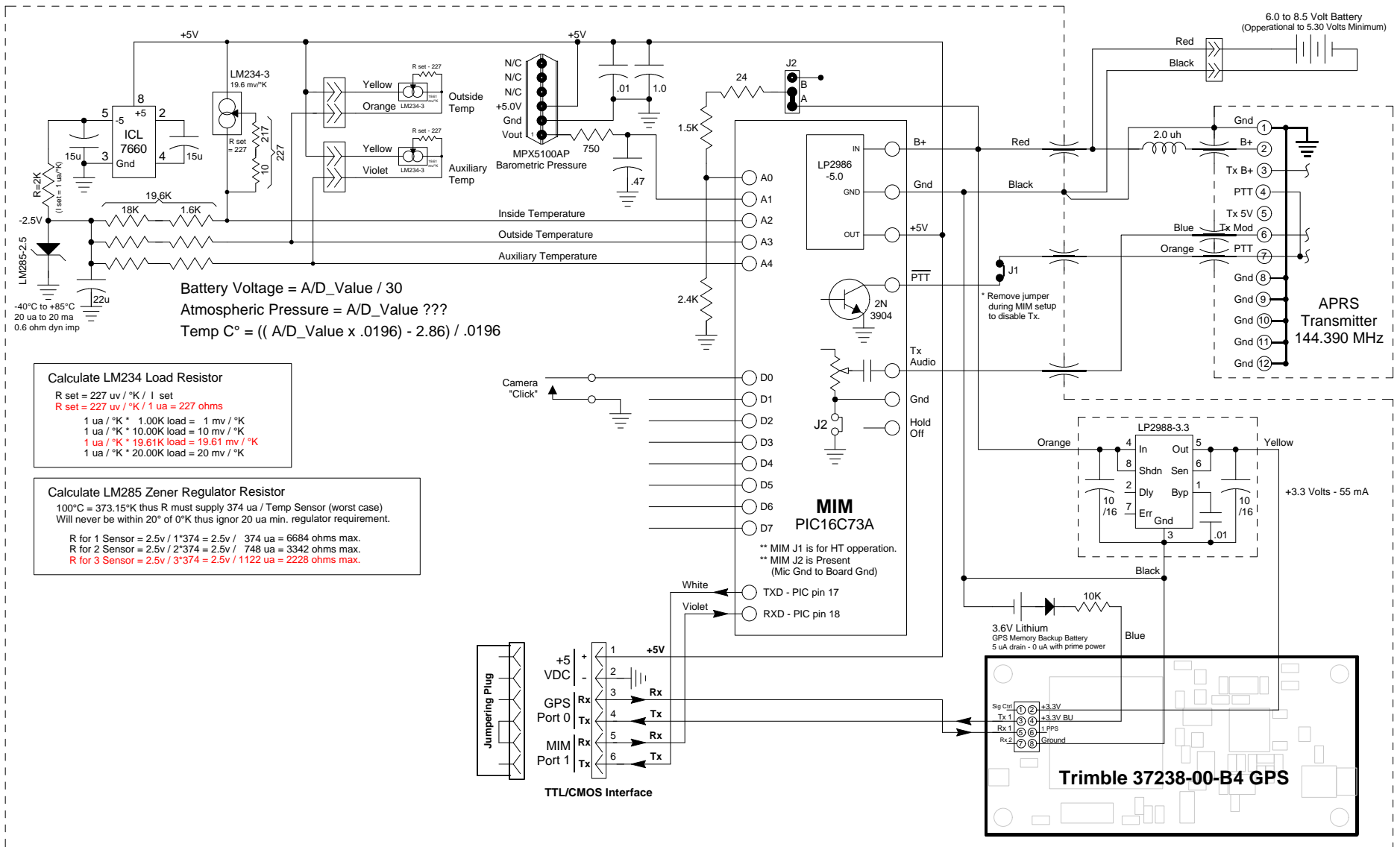
BEAR 2 Tracker Schematic
